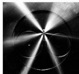
Deposit restricted diesel injector spray pattern
